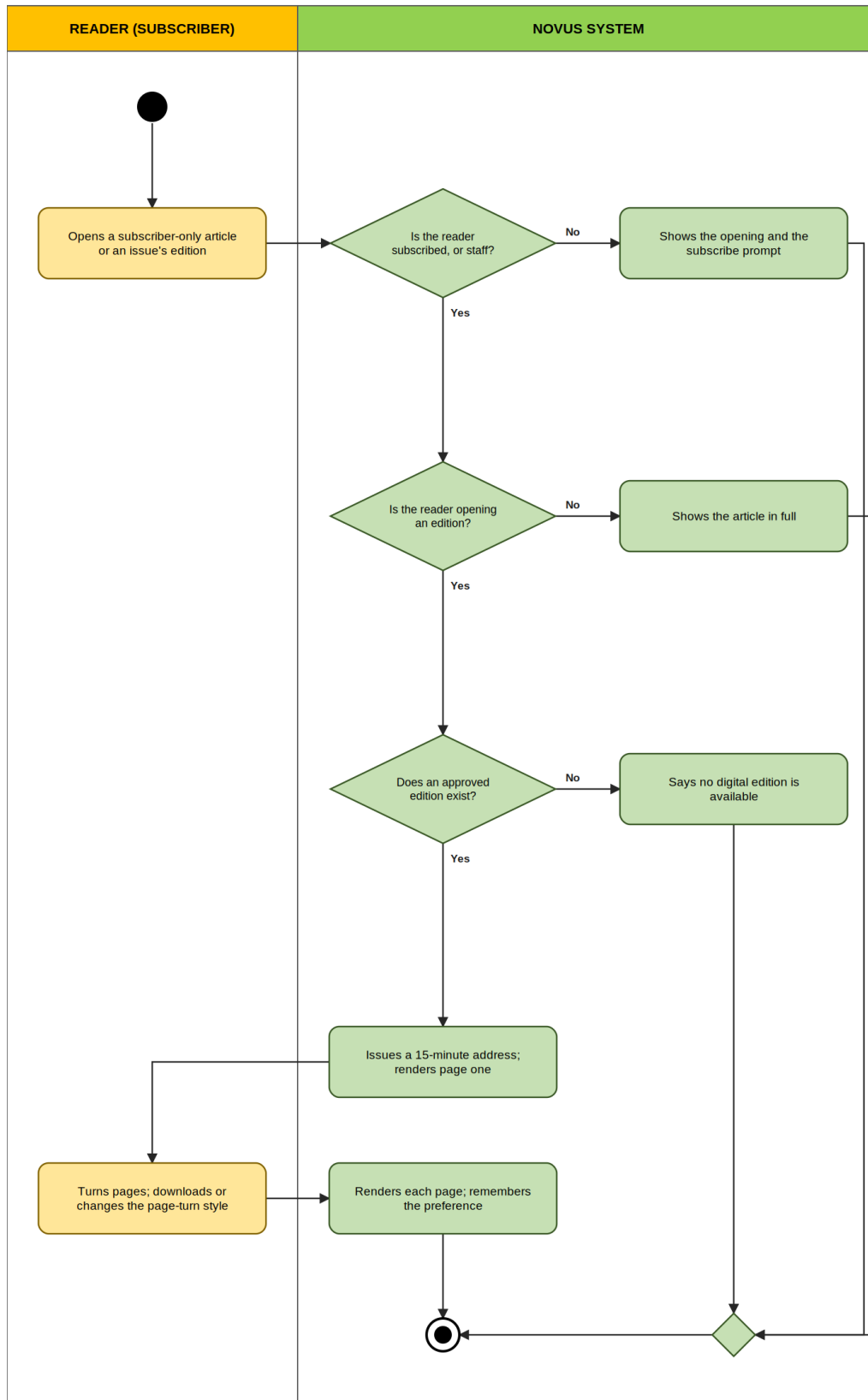
Figure 27 UC-4.3.1: Read Subscriber-Only Content
