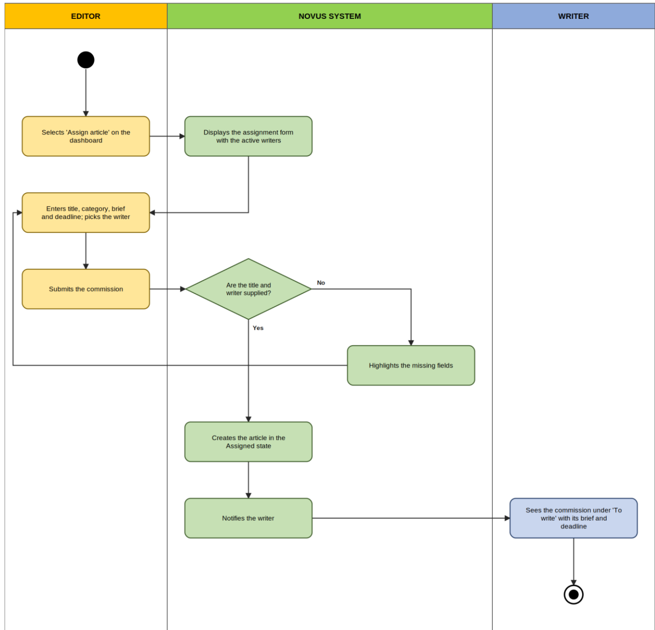
Figure 8 UC-1.1: Commission an article
