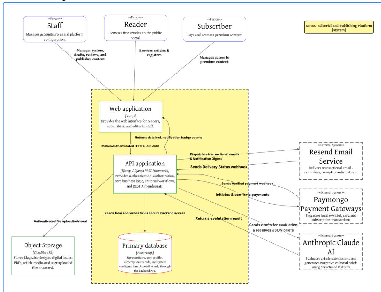
Figure 34 Container Diagram
